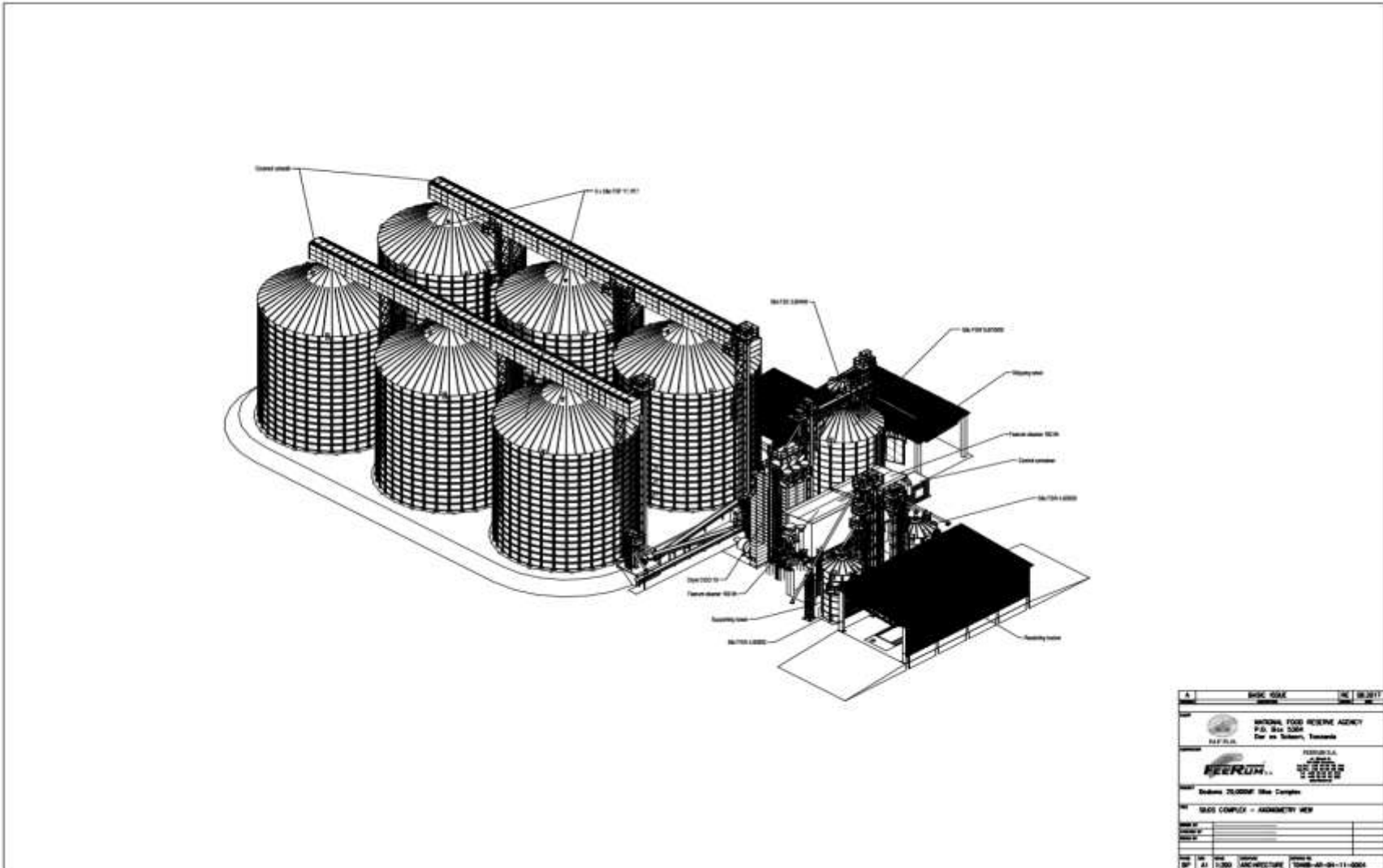
Silo 3 Dimension Layout Plan
